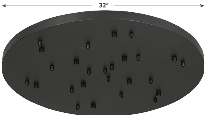
132-BK 32" DIA x 1 1/2" H • UP TO 13 LIGHTS HEAVY METAL • Multi-Port Round Canopy Weight: 33 Lbs.
