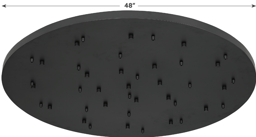
148-BK 48" DIA x 1 1/2" H • UP TO 21 LIGHTS HEAVY METAL • Multi-Port Round Canopy Weight: 60 Lbs.
