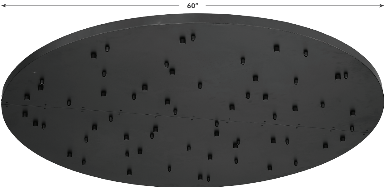
160-BK 60" DIA x 1 1/2" H • UP TO 31 LIGHTS HEAVY METAL • Multi-Port Round Canopy Weight: 108 Lbs.
