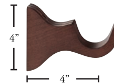
MAD251-XX Wood Bracket
