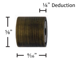
MAR216-XX Inside Mount Bracket
