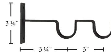
TOR234-XX York Double Open Bracket
