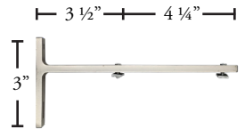
AVA223-XX Double Wall Bracket
