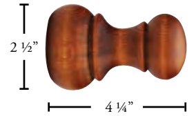
CAM155-XX Campina Finial $43.31 ea. unfinished $64.41 ea. finished
