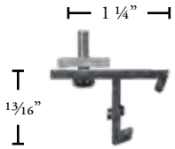
BRU221-XX Ceiling Bracket $28.12 ea.
