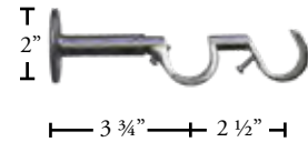
PRA241-SS Juve Double Wall Bracket Adjustable to 5 1/4" $61.63 ea.
