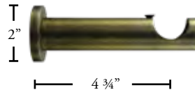
NCA238-XX Extended Wall Bracket $67.13 ea.
