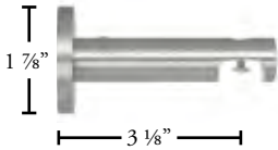
GAL242-SS Single Wall Bracket $106.00 ea.
